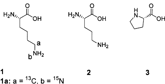
Figure 1. L-lysine ( 1 ), L-ornithine ( 2 ) and L-proline ( 3 )
