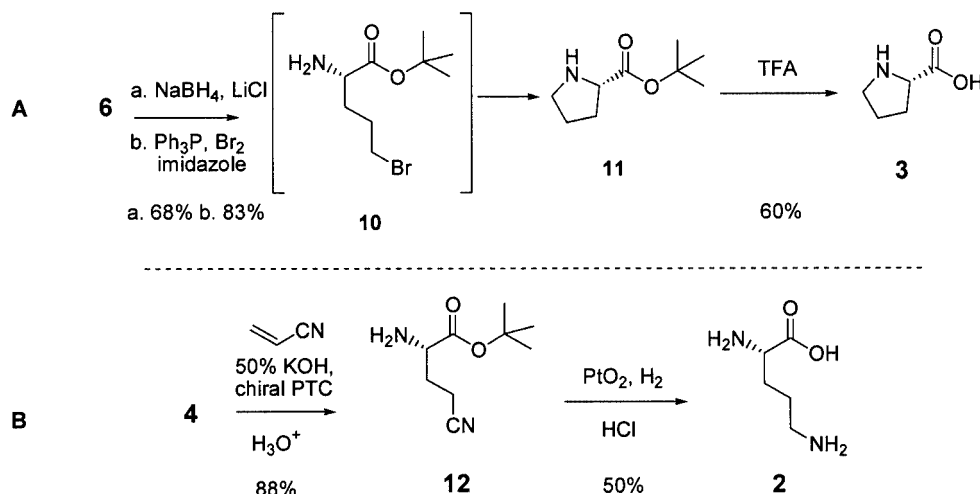
Scheme 2. A – The synthesis of L-proline ( 3 ) starting from chiral tert -butyl methyl glutamate ( 6 ); B – the synthesis of L-ornithine ( 2 ) starting from achiral glycinate 4
